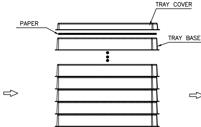
2. TRAYS OVERLAY: (THE NEXT TRAY NEED ROTATE 180 DEGREE AND PUT IT ON PREVIOUS TRAY.) (相邻两个吸塑间水平方向成180度摆放)
