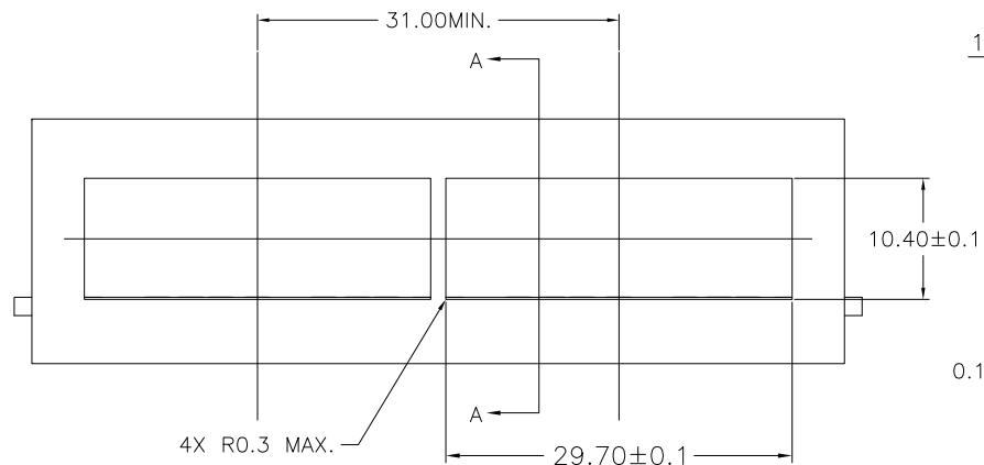
RECOMMENDED BEZEL DESIGN SINGLE SIDED APPLICATIONS
