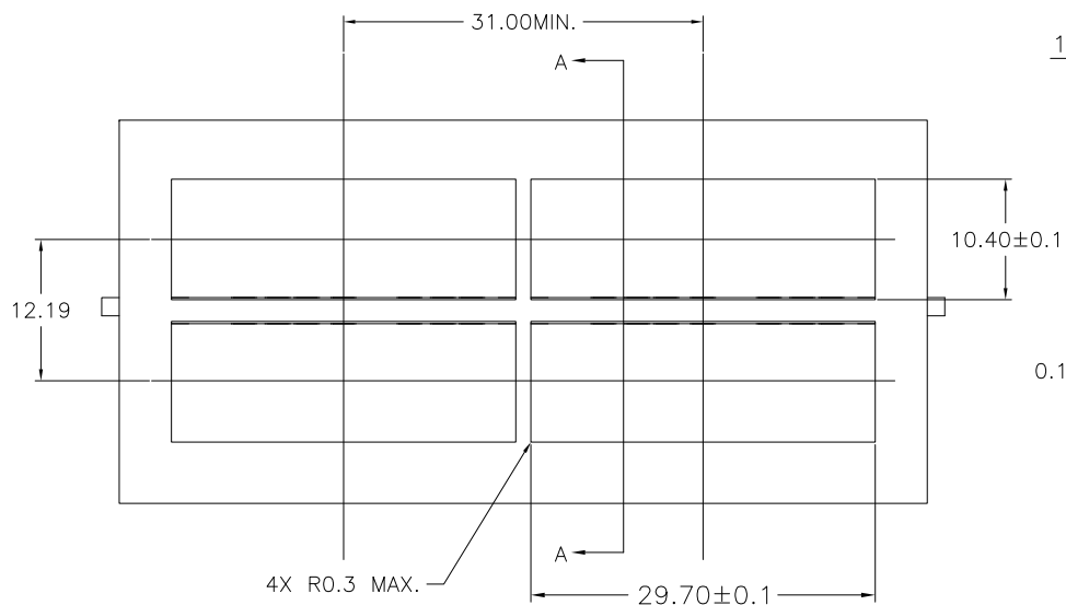
RECOMMENDED BEZEL DESIGN BELLY TO BELLY APPLICATIONS
