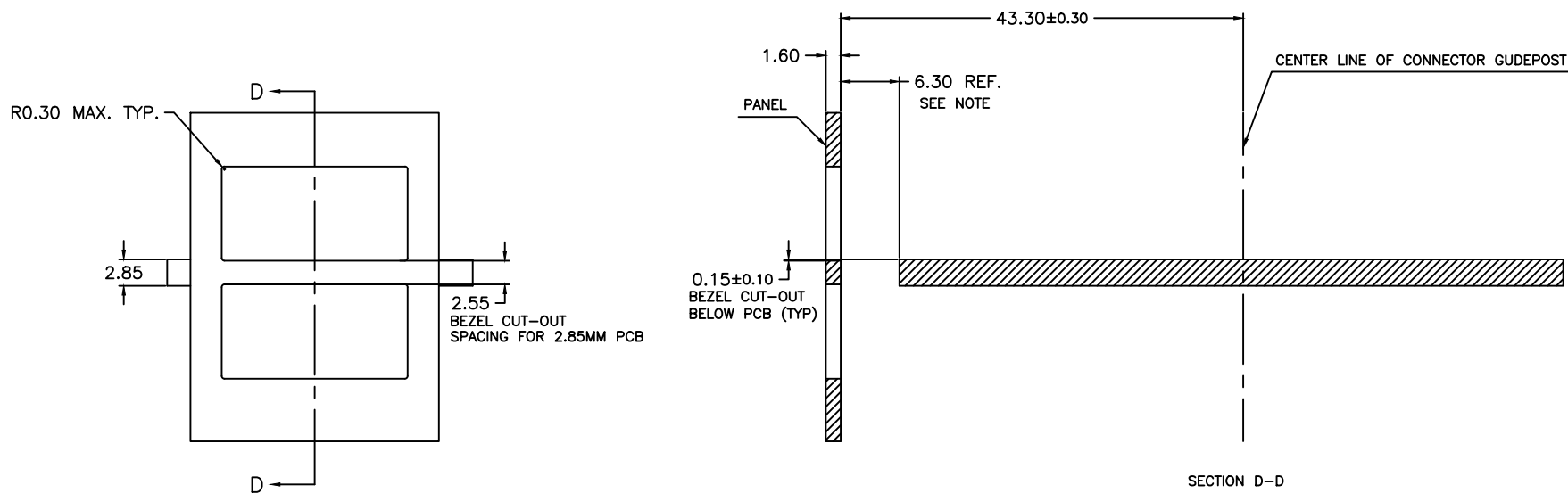
RECOMMENDED BELLY-TO-BELLY MOUNTING DESIGN
