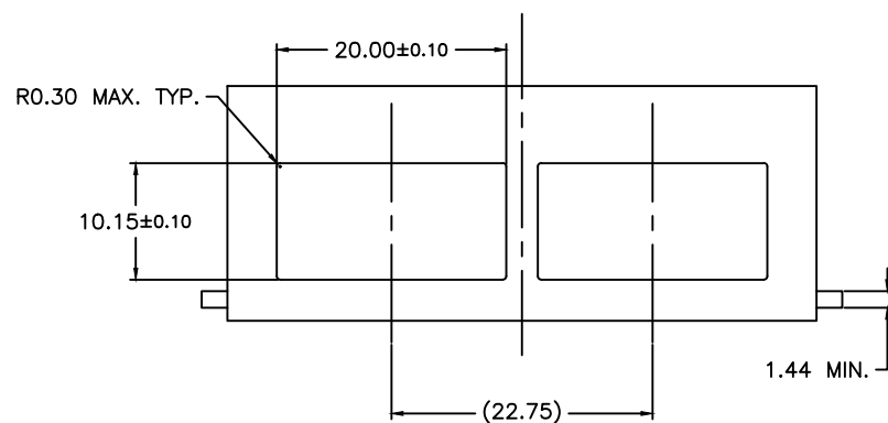
RECOMMENDED SINGLE SIDE MOUNTING DESIGN
