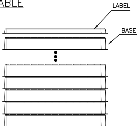
2. TRAYS OVERLAY: (THE NEXT TRAY NEED ROTATE 180 DEGREE AND PUT IT ON PREVIOUS TRAY.) (相邻两个吸塑间水平方向成180度摆放)
