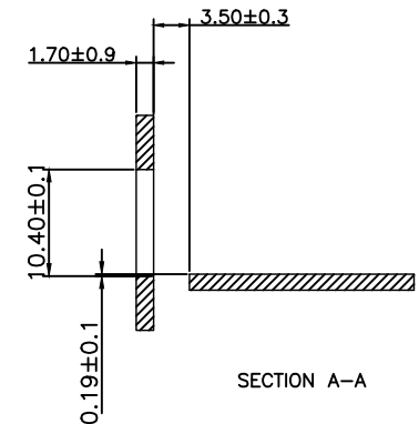
RECOMMENDED BEZEL DESIGN
