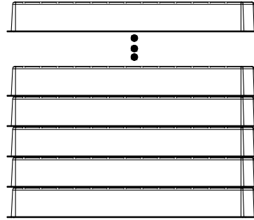
2. 5PCS TRAYS OVERLAY: (THE NEXT TRAY NEED ROTATE 180 DEGREE AND PUT IT ON PREVIOUS TRAY.) (相邻两个吸塑间水平方向成180度摆放)
