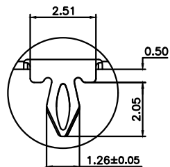
DETAIL A SCALE 5:1
