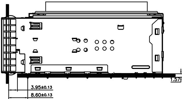
SECTION U-U
