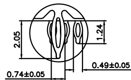
DETAIL B SCALE 5:1
