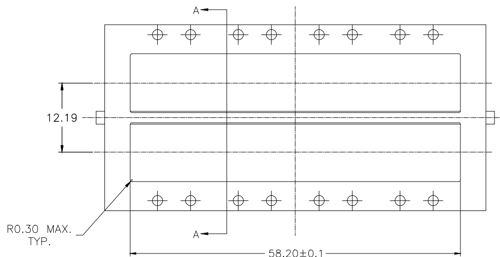
RECOMMENDED BEZEL DESIGN BELLY TO BELLY APPLICATIONS
