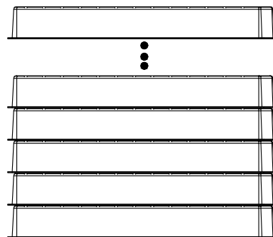
2. 10PCS TRAYS OVERLAY: (THE NEXT TRAY NEED ROTATE 180 DEGREE AND PUT IT ON PREVIOUS TRAY.) (相邻两个吸塑间水平方向成180度摆放)
