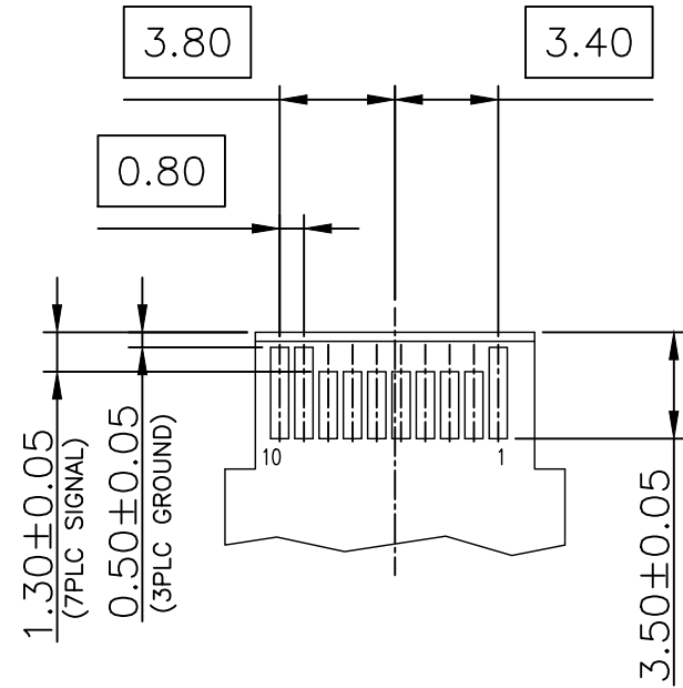
BOTTOM VIEW OF BOARD
