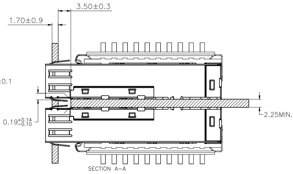
RECOMMENDED BEZEL DESIGN SINGLE SIDED APPLICATIONS
