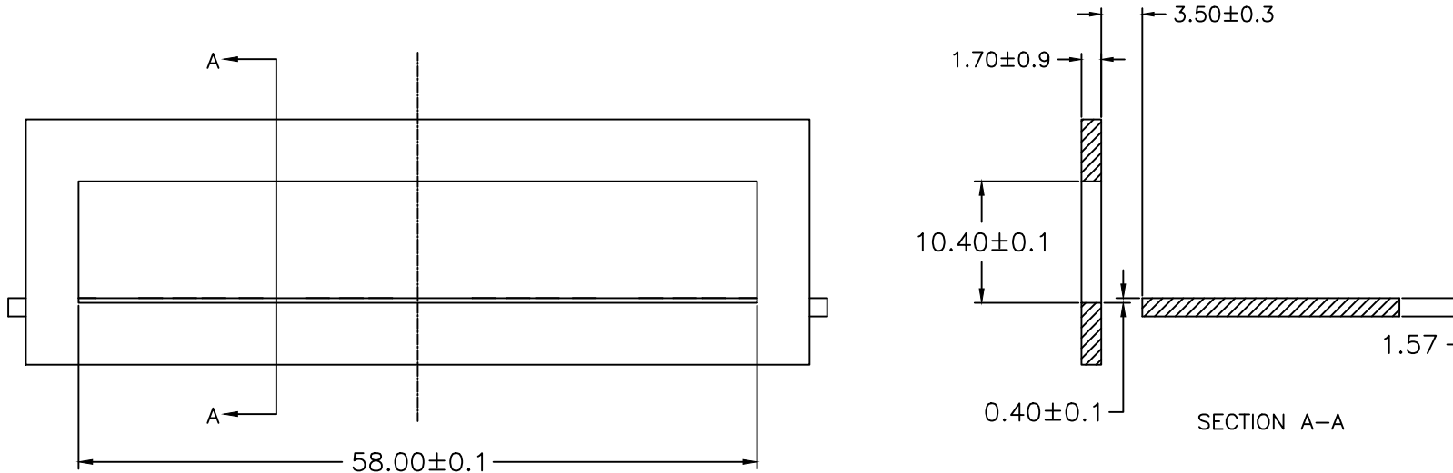
RECOMMENDED BEZEL DESIGN
