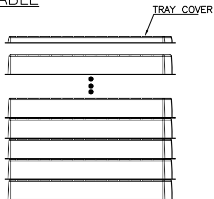
2. TRAYS OVERLAY: (THE NEXT TRAY NEED ROTATE 180 DEGREE AND PUT IT ON PREVIOUS TRAY.) (相邻两个吸塑间水平方向成180度摆放)
