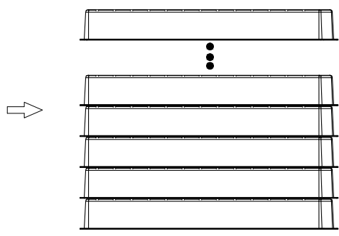
2. 4PCS TRAYS OVERLAY: (THE NEXT TRAY NEED ROTATE 180 DEGREE AND PUT IT ON PREVIOUS TRAY.) (相邻两个吸塑间水平方向成180度摆放)
