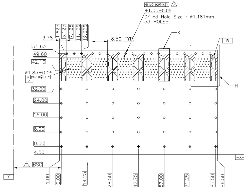
RECOMMENDED PCB CONFIGURATION
