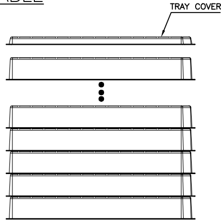
2. TRAYS OVERLAY: (THE NEXT TRAY NEED ROTATE 180 DEGREE AND PUT IT ON PREVIOUS TRAY.) (相邻两个吸塑间水平方向成180度摆放)
