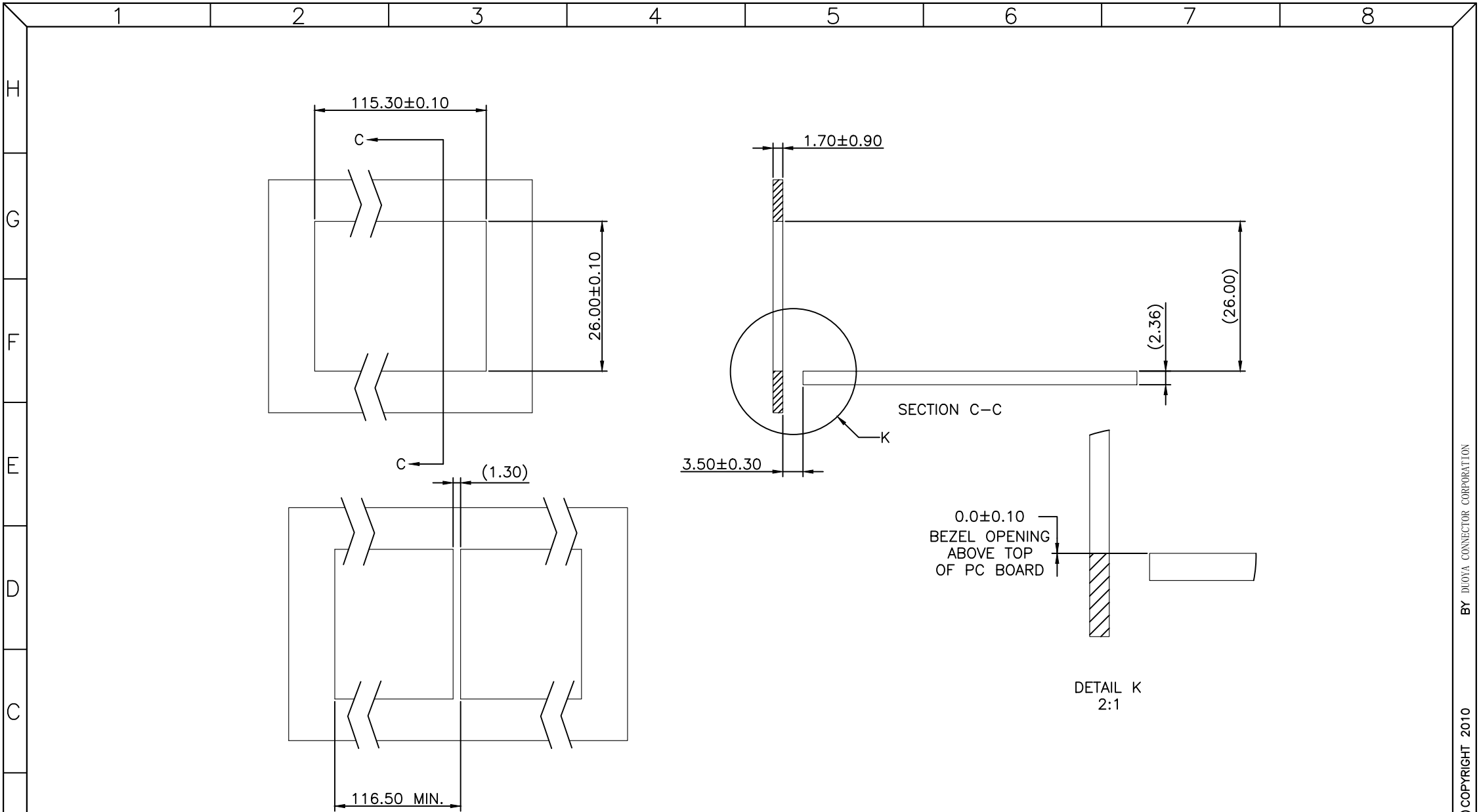
RECOMMENDED BEZEL DESIGN
