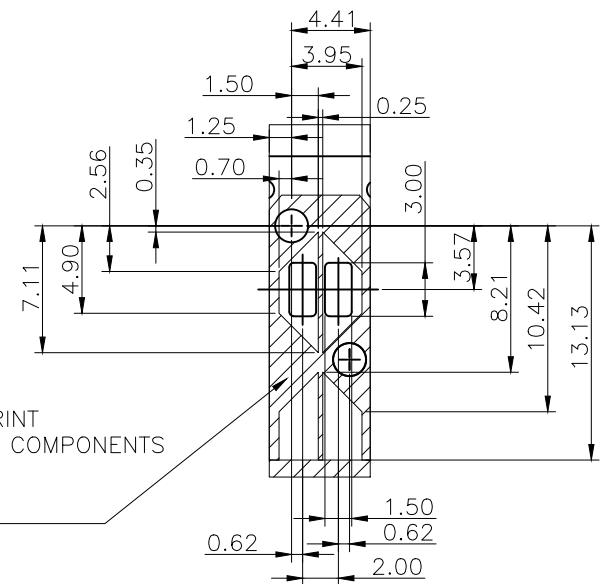
DETAIL LIGHT PIPE LOCATION AND OTHER ZONES DETAIL K 2:1
