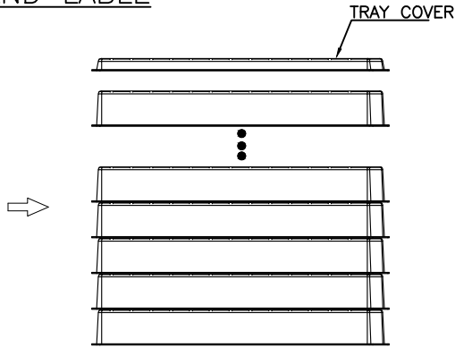
2. TRAYS OVERLAY: (THE NEXT TRAY NEED ROTATE 180 DEGREE AND PUT IT ON PREVIOUS TRAY.) (相邻两个吸塑间水平方向成180度摆放)
