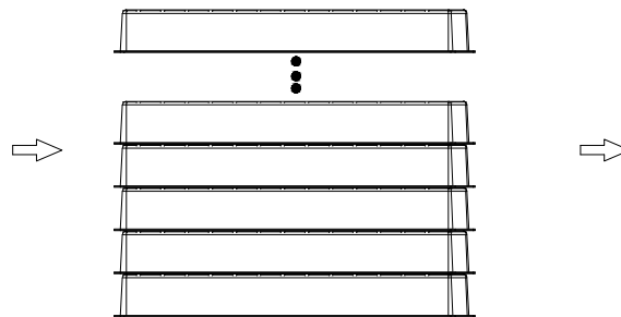
2. 5PCS TRAYS OVERLAY: (THE NEXT TRAY NEED ROTATE 180 DEGREE AND PUT IT ON PREVIOUS TRAY.) (相邻两个吸塑间水平方向成180度摆放)
