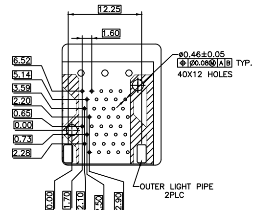
DETAIL H 2:1 RECOMMENDED PCB CONFIGURATION
