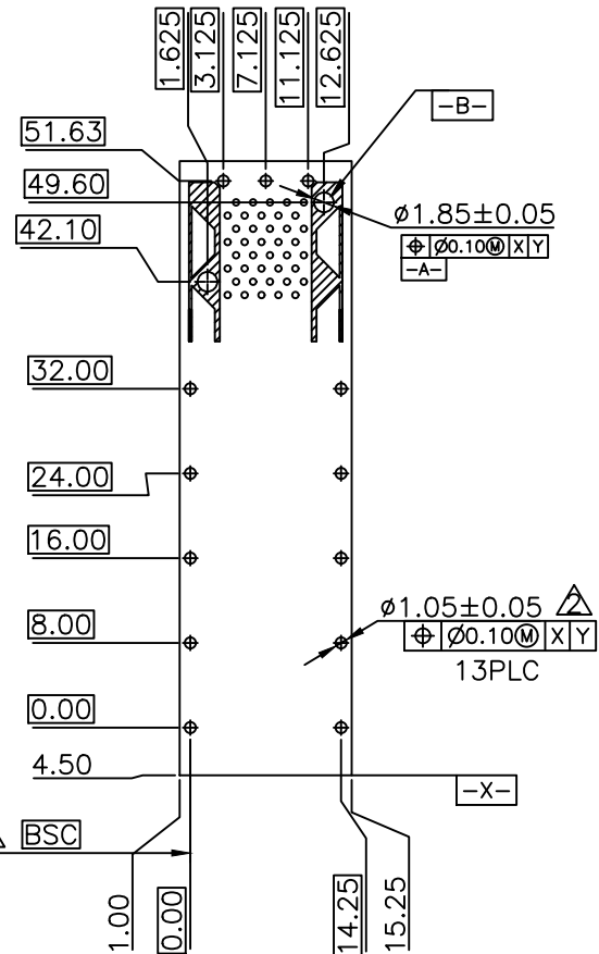
RECOMMENDED PCB CONFIGURATION
