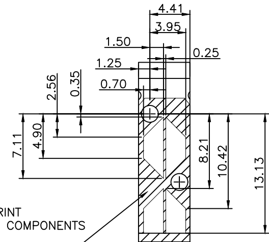
DETAIL LIGHT PIPE LOCATION AND OTHER ZONES DETAIL K 2:1
