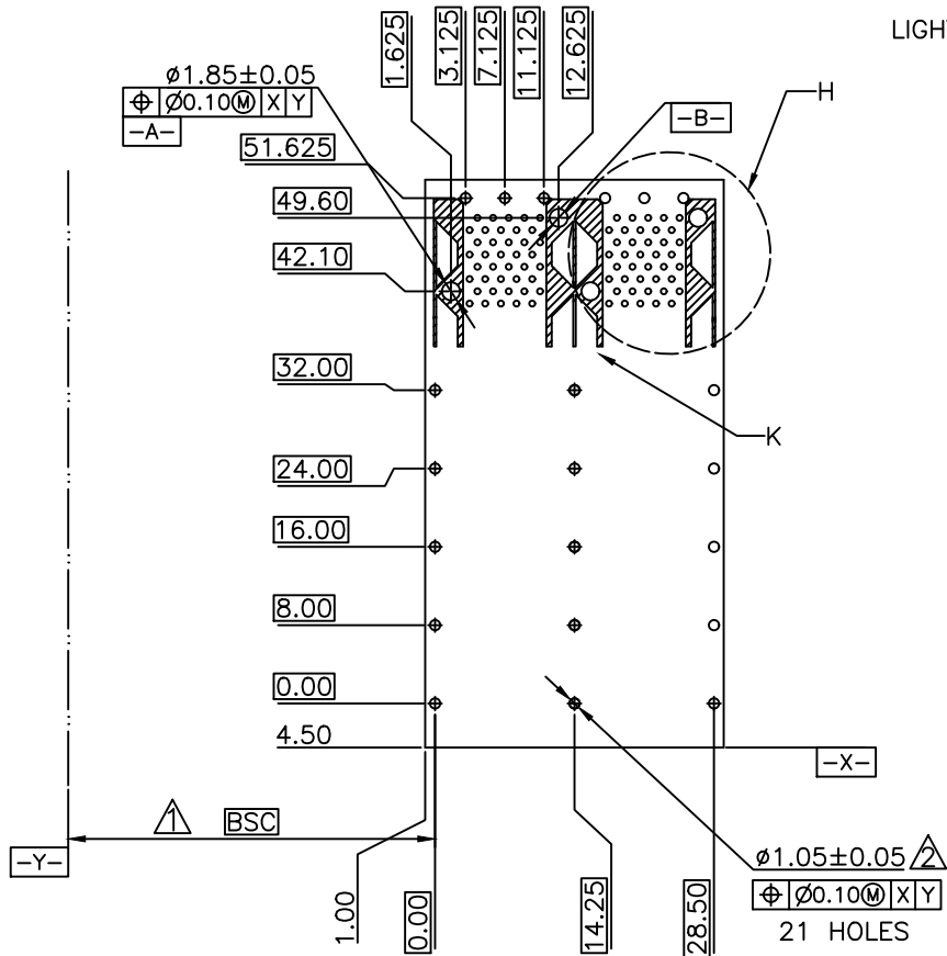
RECOMMENDED PCB CONFIGURATION
