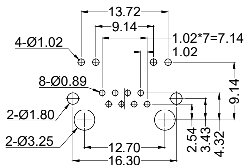
RECOMMENDED PCB LAYOUT (COMPONENT SIDE VIEW) TOLERANCE:±0.05
