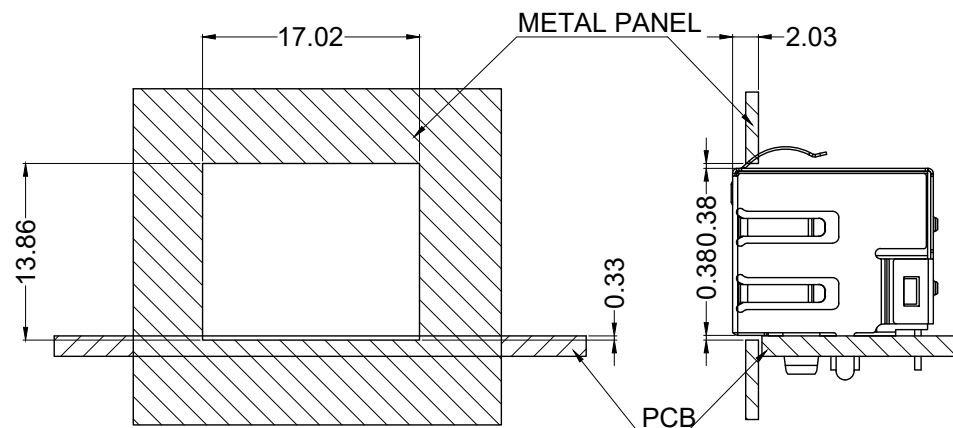
ADD RECOMMENDED PANEL OPENING SIZE
