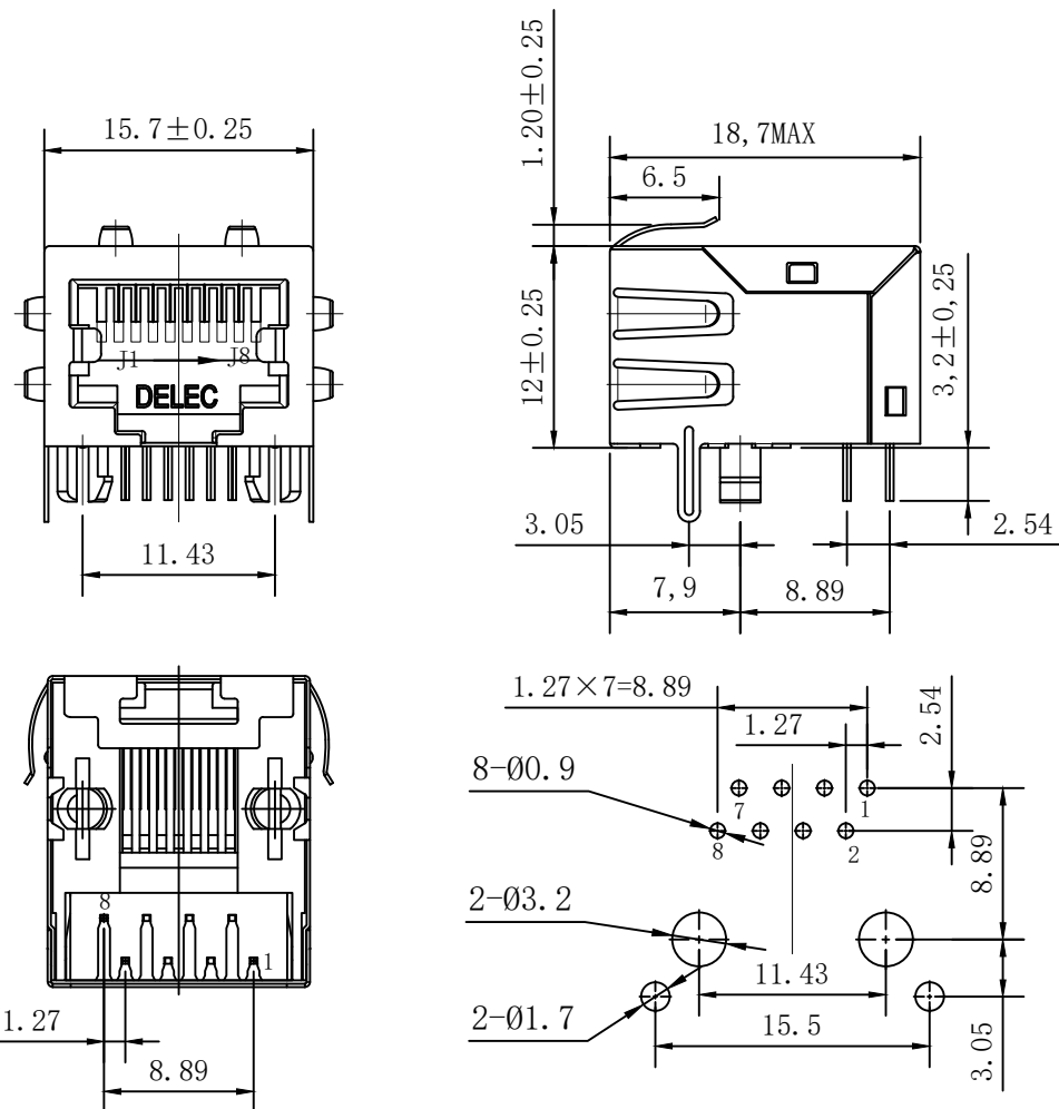
RECOMMENDED PCB LAYOUT (COMPONENT SIDE VIEW)
