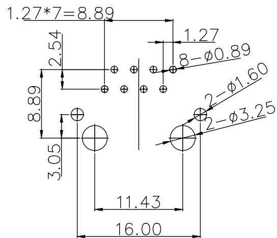
RECOMMENDED PCB LAYOUT (COMPONENT SIDE VIEW) TOLERANCE: \pm 0.05
