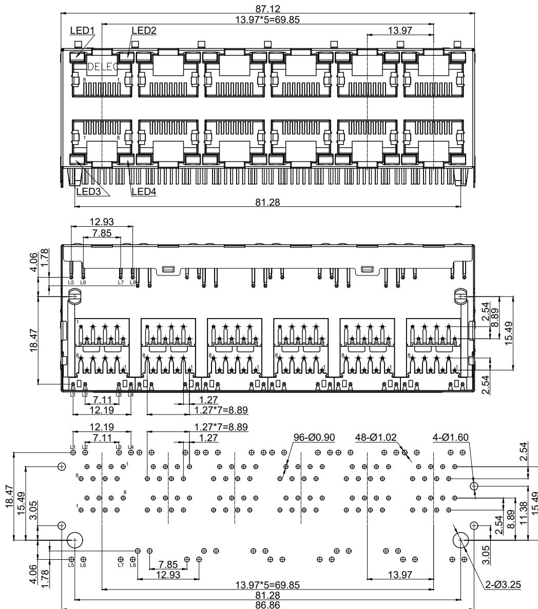
RECOMMENDED PCB LAYOUT (COMPONENT SIDE VIEW)
