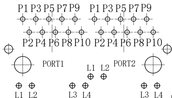
PIN NUMBER ASSIGN (COMPONENT SIDE VIEW)
