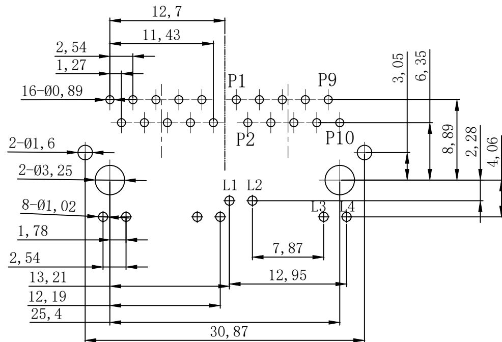
RECOMMENDED PCB LAYOUT (COMPONENT SIDE VIEW) TOLERANCE: \pm 0.08
