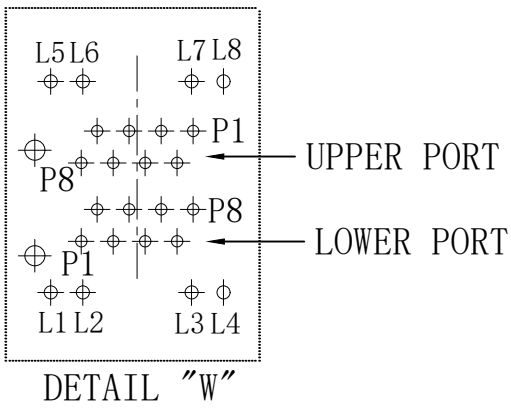
RECOMMENDED PCB LAYOUT (COMPONENT SIDE VIEW)
