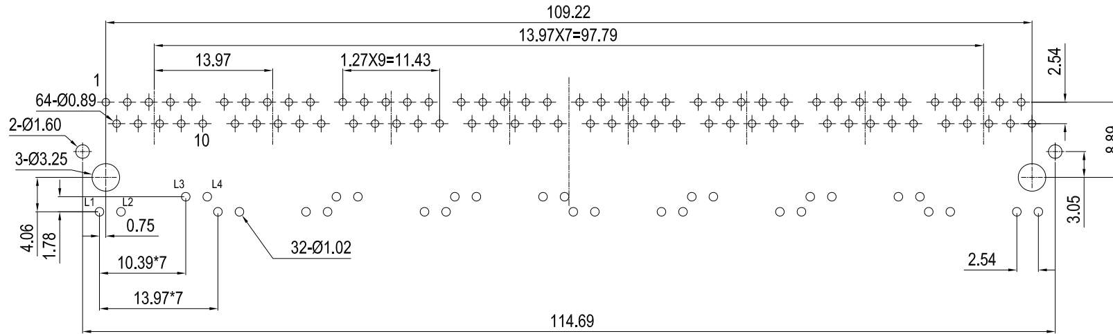
RECOMMENDED PCB LAYOUT (COMPONENT SIDE VIEW)
