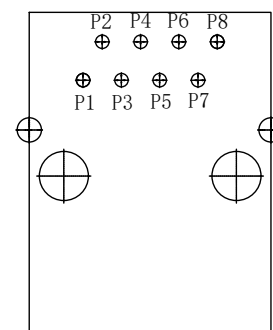
PIN NUMBER ASSIGN (COMPONENT SIDE VIEW)
