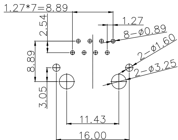
RECOMMENDED PCB LAYOUT (COMPONENT SIDE VIEW) TOLERANCE: \pm 0.05
